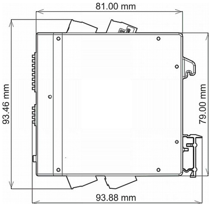
Fig.1: LP21/LP22 side view
